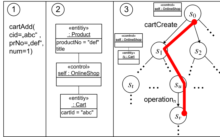
Fig. 5. Three steps of test case generation
