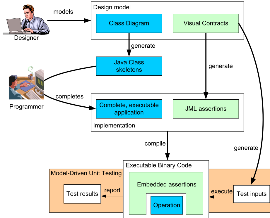
Fig. 1. Overview of the testing approach
