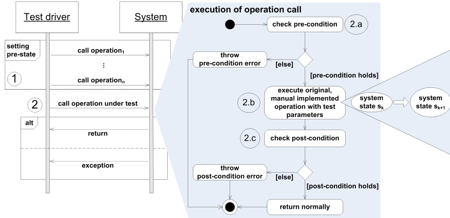
Fig. 6. Run-time behavior of test execution
