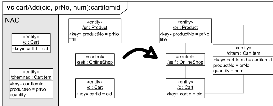
Fig. 4. Visual contract for operation cartAdd
